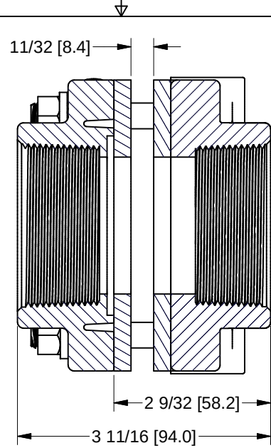
SECTION B-B SCALE 1
