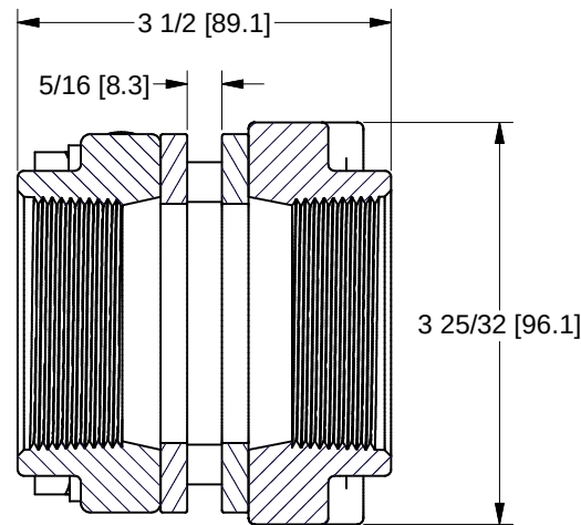
SECTION B-B SCALE 1
