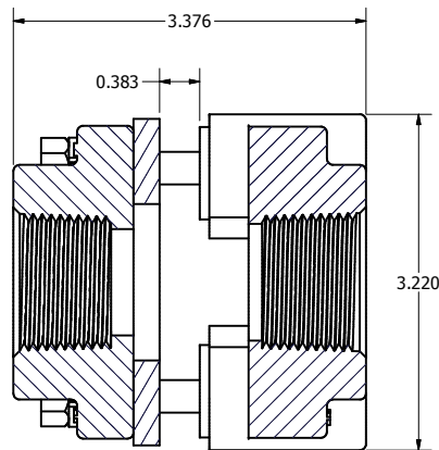
SECTION E-E SCALE 1 : 1
